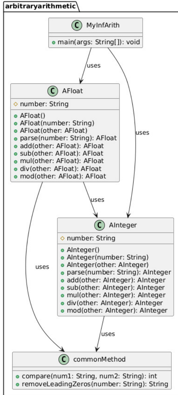
Figure: Class relationships and design of the Arbitrary Precision Arithmetic Library.
